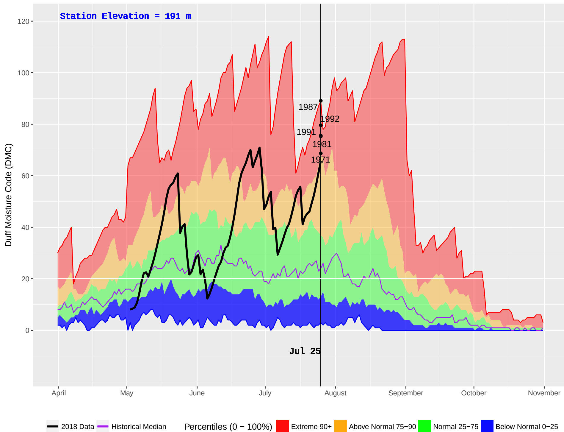
NASS CAMP (427) : Historical (1970–2016) and Current (2018) Noon Duff Moisture Code (DMC)
